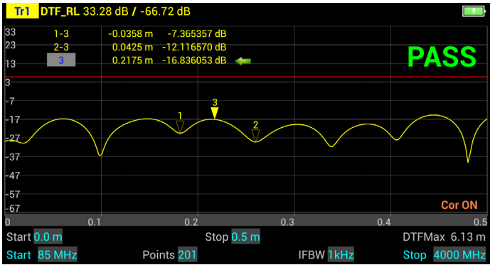
Figure 19 Highlighted Markers
