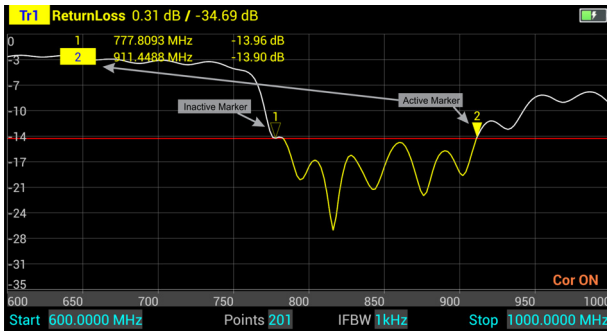
Figure 17 Marker Examples
