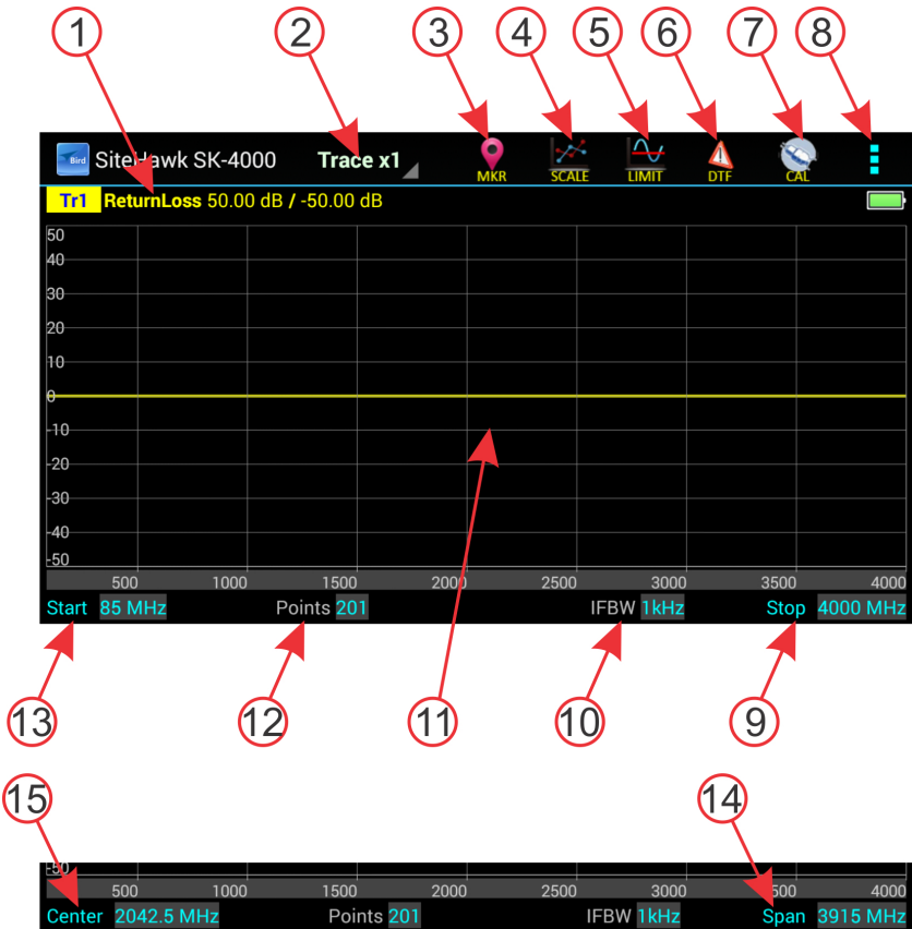
Figure 2 User Interface Description (Match Measurement Mode)
