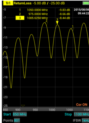
Figure 21 Marker 3 Peak Search
